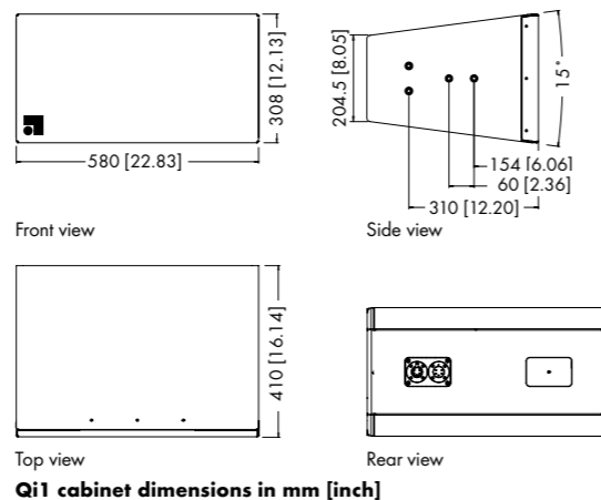
Qi1 cabinet dimensions in mm [inch]
