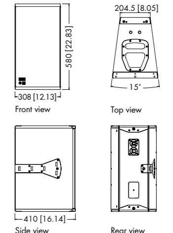
Q7 cabinet dimensions in mm [inch]
