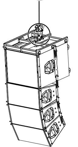
Q1/Q-SUB array with Z5159 Q Flying frame Z5154 Q Rigging set Z5147 Rota clamp Z5160 Q Load adapter
