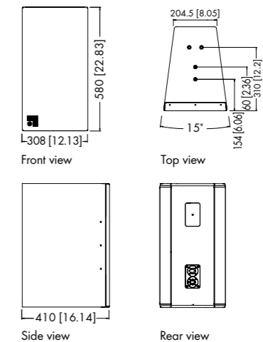
Qi7 cabinet dimensions in mm [inch]
