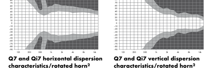
Q7 and Qi7 horizontal dispersion characteristics 2
