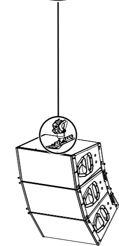
Q1 array with Z5156 Q Flying adapter Z5154 Q Rigging set Z5147 Rota clamp
