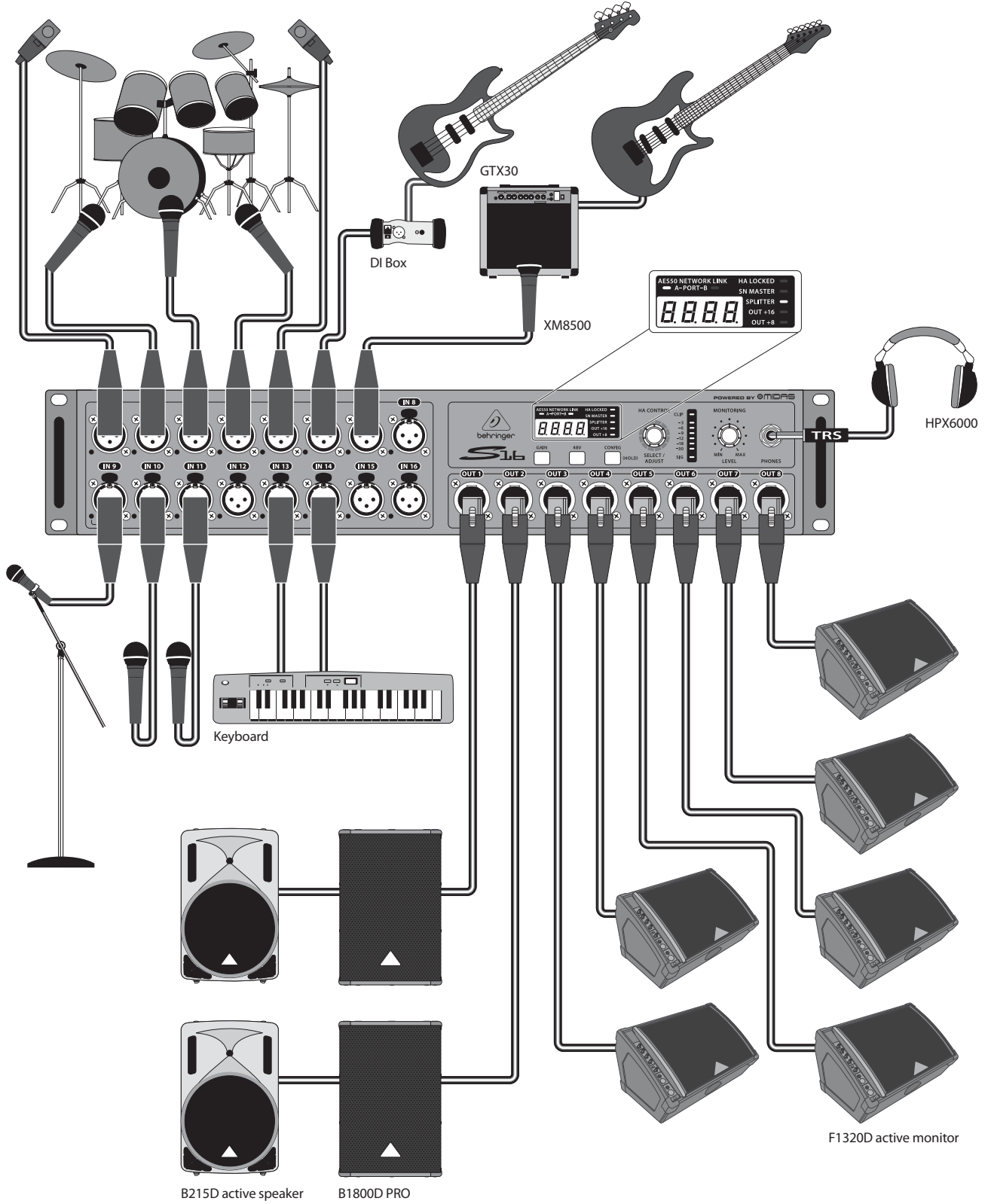
Common connections
